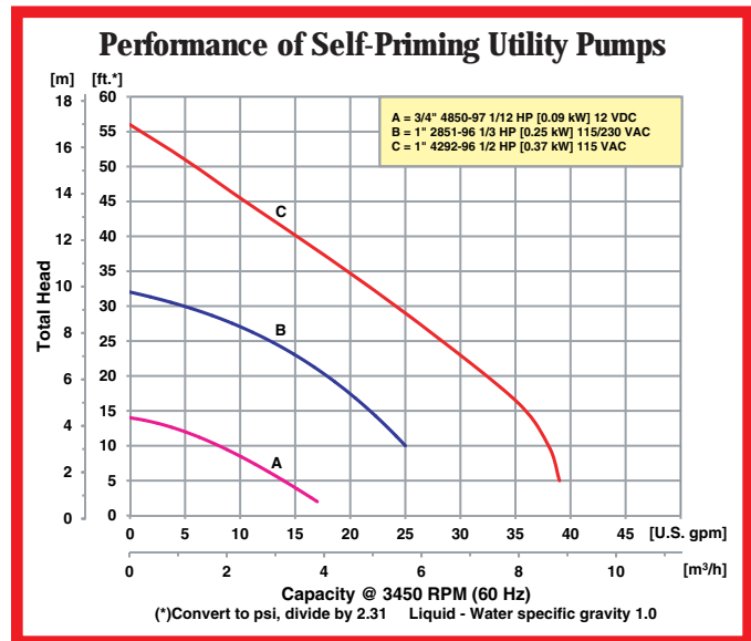
Model 4850-97 Cast Bronze
